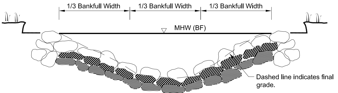
Figure 8 Cross Vane Details
